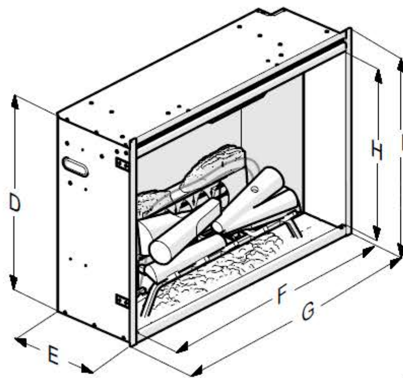
Firebox Dimensions
