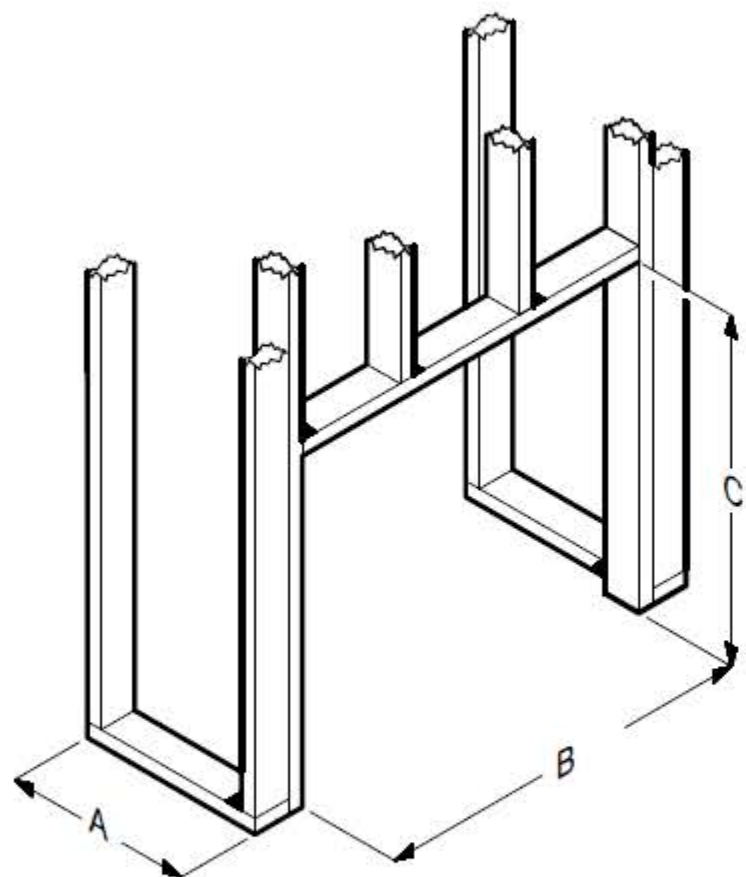
Rough-In Framing Dimensions
